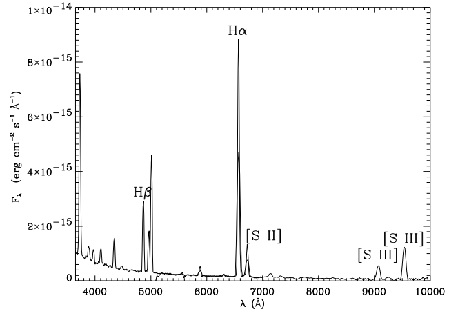
Fig. 2. Combined spectrum of the region 53A, B. Notice how smoothly the blue and red part of the spectrum merge. In the overlapping region the difference in resolution is obvious. The most important lines are labeled.
